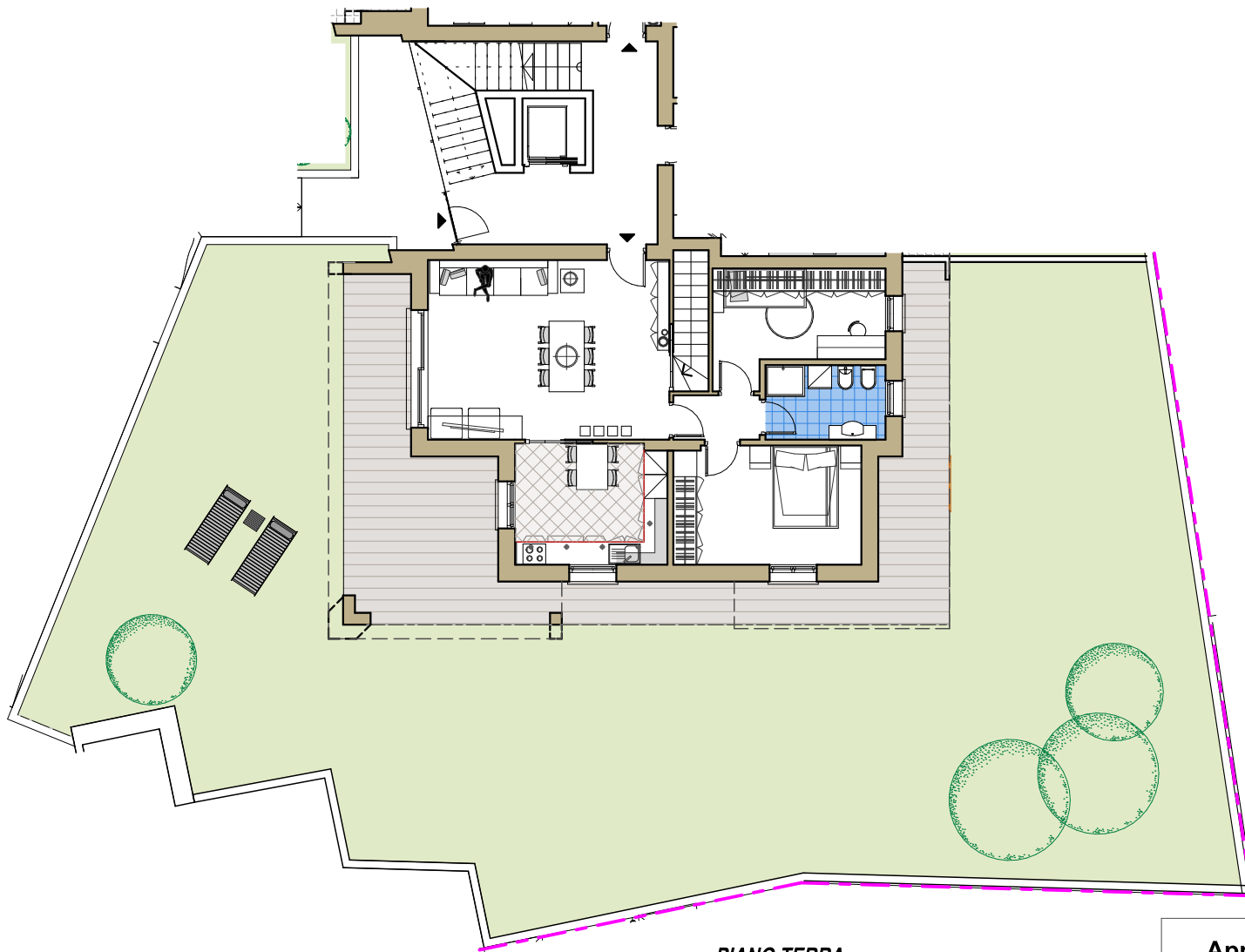
PIANO TERRA
