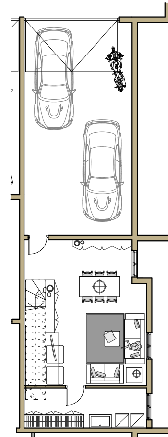
PIANO INTERRATO
